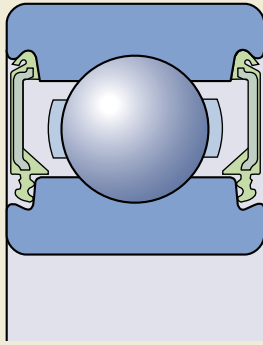
RSH seal design for an outside diameter larger than 25 mm
